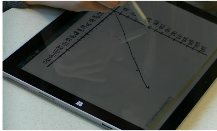
Fig. 34: S1's graph.
